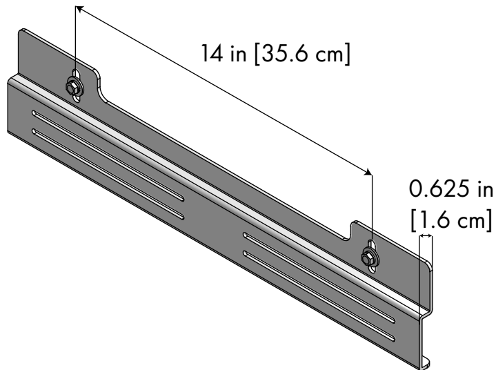
Sound Bar Mount - Isometric View
