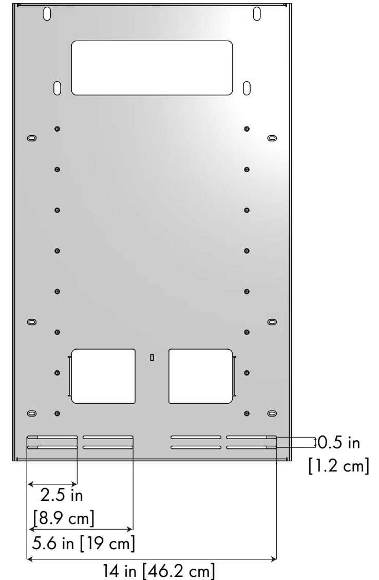
CL-65e Carrier - Front View
