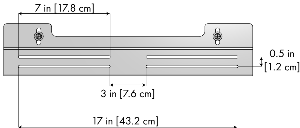
Sound Bar Mount - Front View
